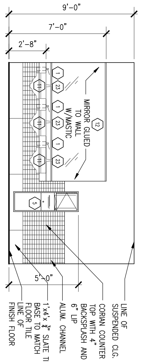
07 TOILET ELEVATION SCALE: 1/4" = 1'-0"
